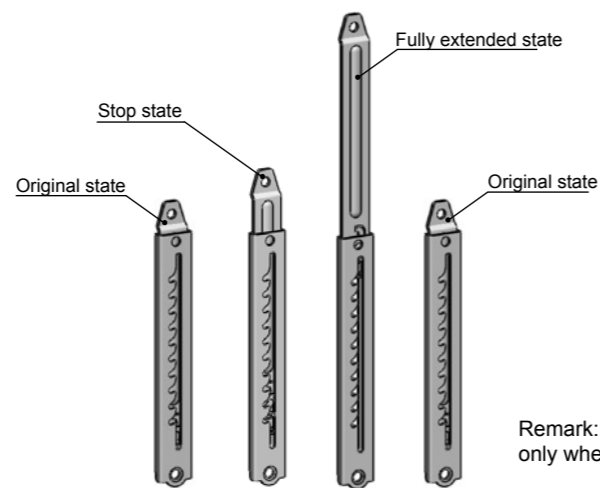
Different states of telescopic cover stay
