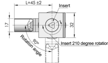
Unadjustable type
