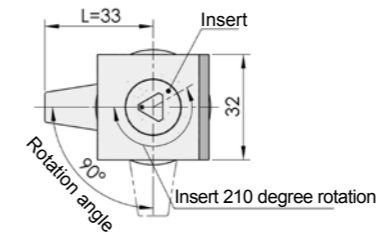
Adjustable type
